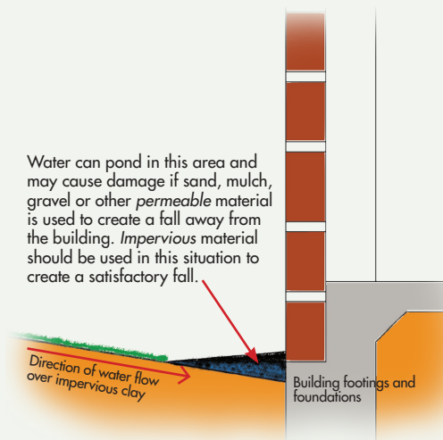
UNSATISFACTORY METHOD FOR CREATING SURFACE FALL AWAY FROM DWELLING
