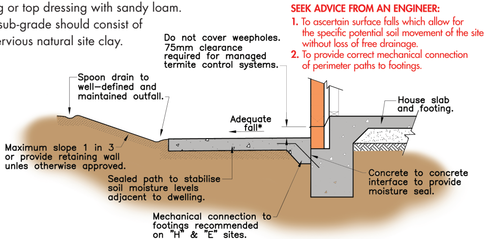
RECOMMENDED DRAINAGE AND MAINTENANCE ADJACENT TO DWELLING
